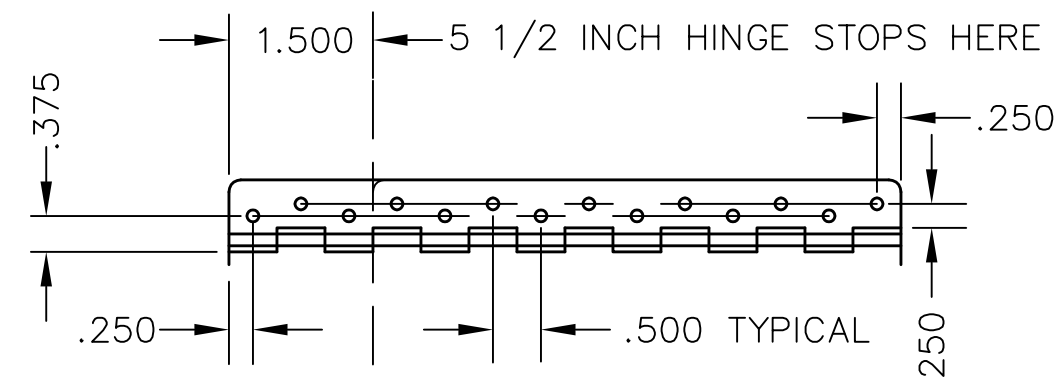
VIEW A: HINGE DRILL DIMENSIONS(SEE TEMPLATE) BOTH SIDES OF HINGE TYPICAL
